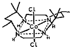
Structure IV. trans -[Co(tetb)Cl 2 ] +
