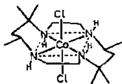
Structure III. trans -[Co(teta)Cl 2 ] +
