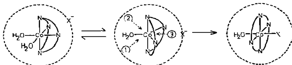
Fig.4. Steric course for the unimolecular anation of \text{cis-[Co(tetb)(OH}_2)_2]^{3+} .
