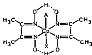
Structure V. trans - [Co(DH)_2AX]
